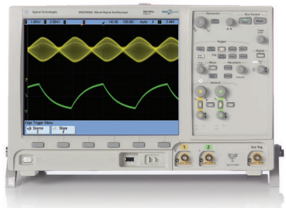
InfiniiVision 7000A Series 2-channel model
